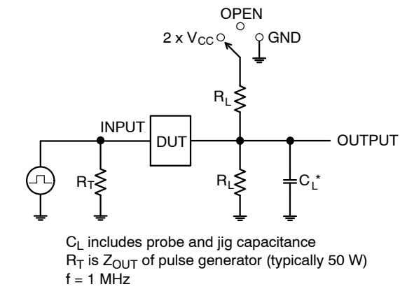
Figure 5. Test Circuit
