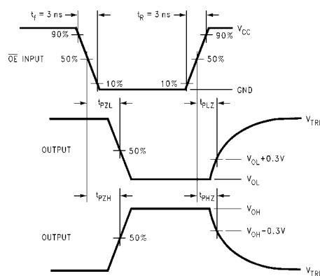
Figure 6. AC Waveforms
