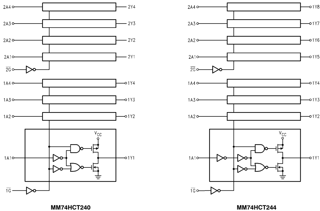
Figure 1. Logic Diagrams
