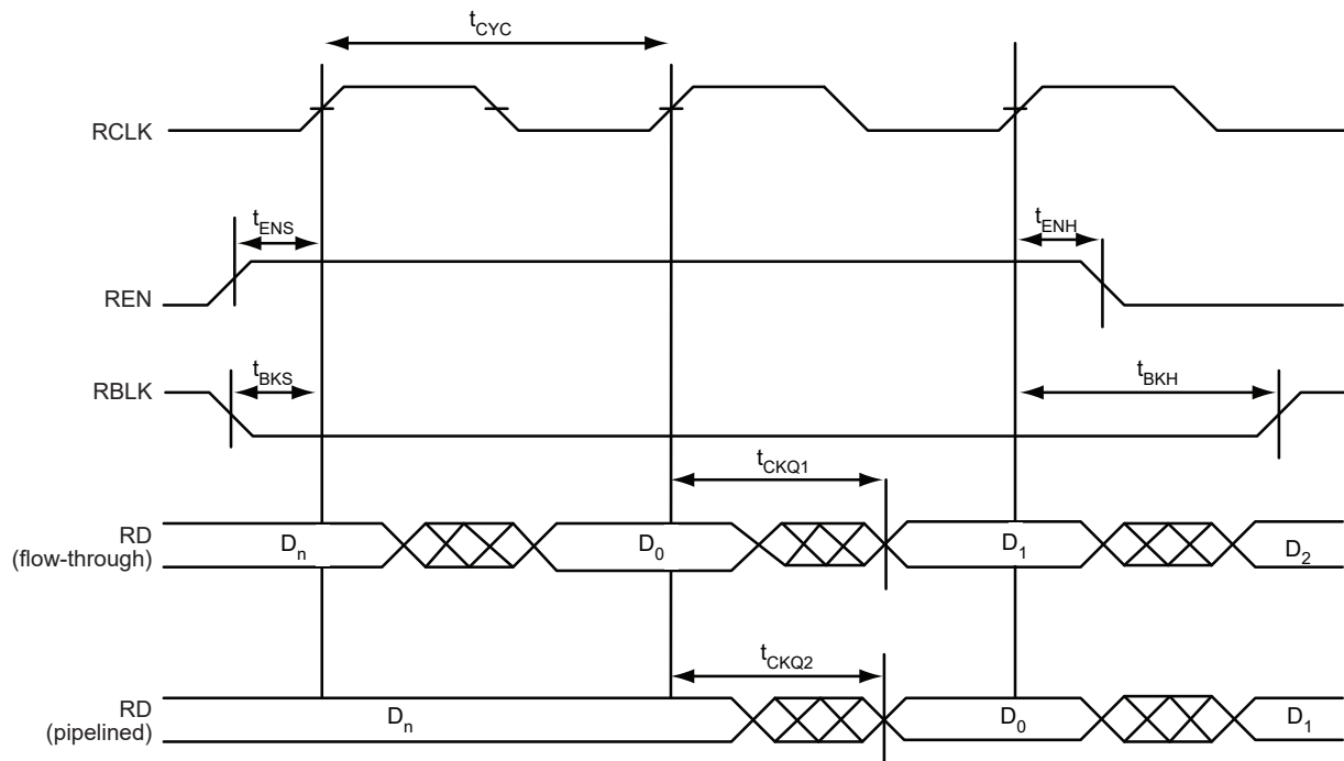
FIGURE 2-47: FIFO READ
