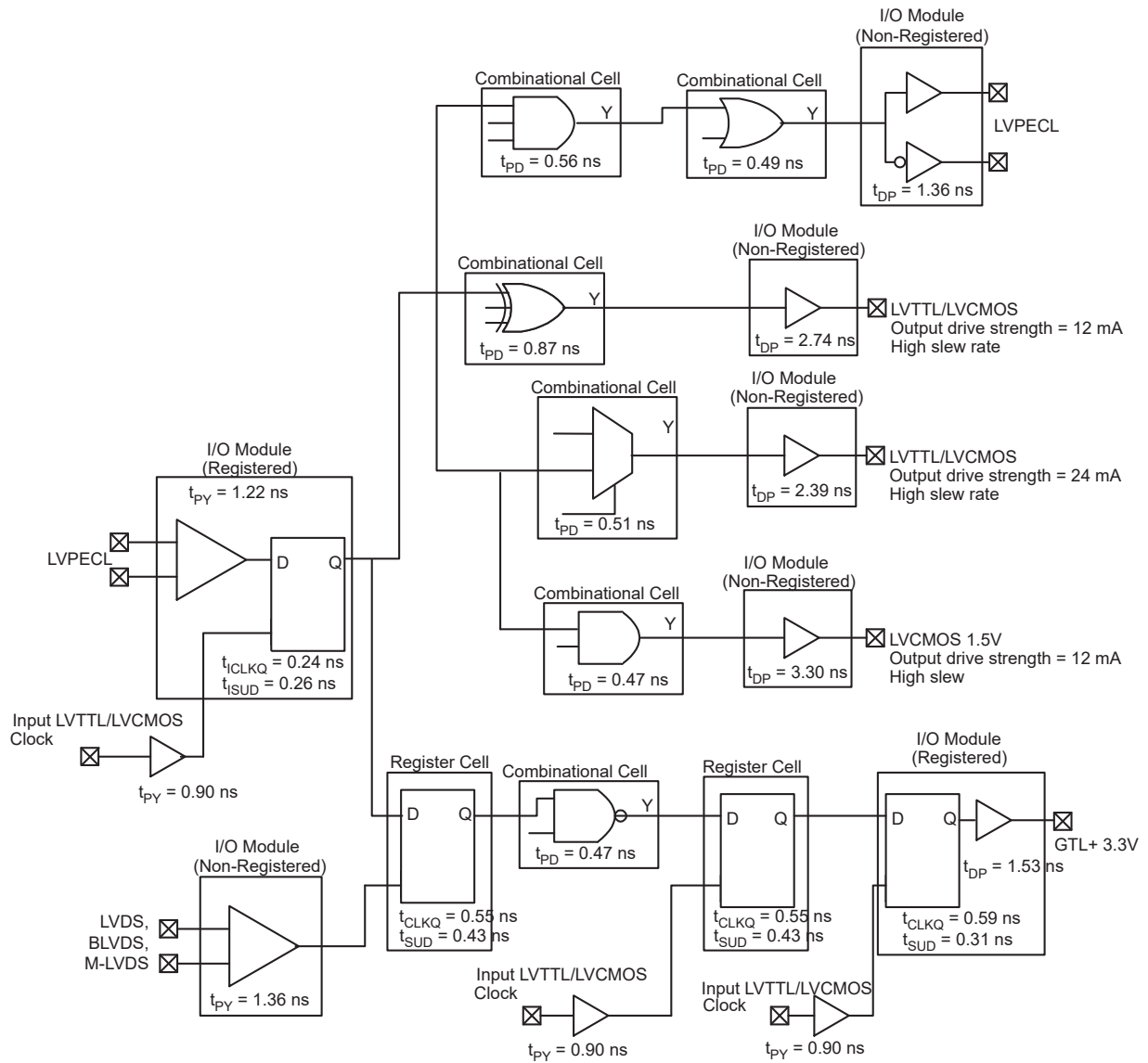
FIGURE 2-2: TIMING MODEL (OPERATING CONDITIONS: -2 SPEED, COMMERCIAL TEMPERATURE RANGE (TJ = 70°C), WORST-CASE VCC = 1.425 V)
