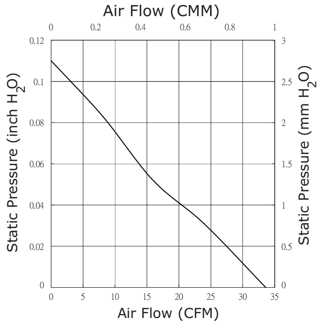
CFM-8015V-227-320
