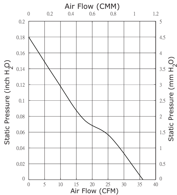
CFM-8020V-142-450
