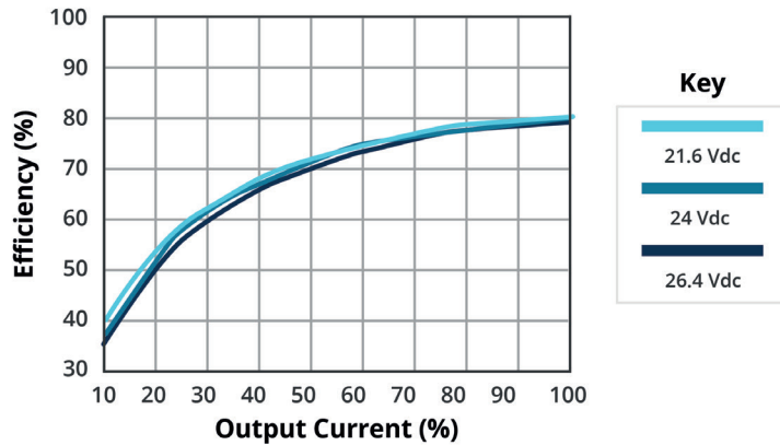
EFFICIENCY VS OUTPUT LOAD PCSA1-S24-S12-S
