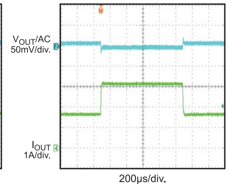
Transient Response
