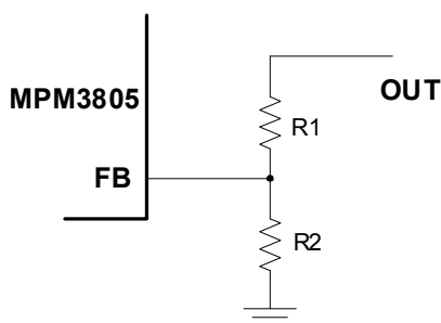
Figure 2: Feedback Network
