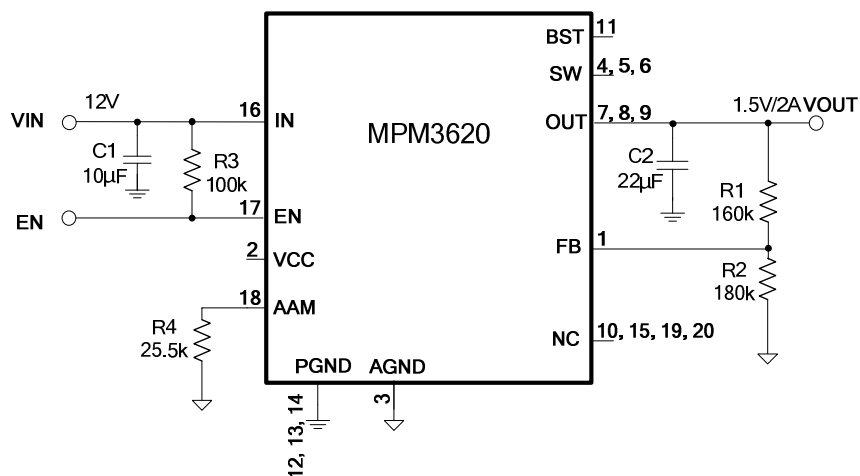
Figure 16. V_{OUT}=1.5V , I_{OUT}=2A
