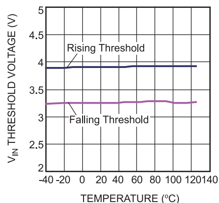
V_{IN} Threshold vs. Temperature EN=5V
