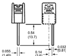
07 Extended Pin
