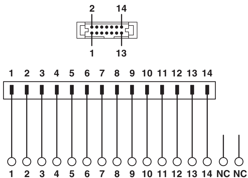
Circuit diagram
