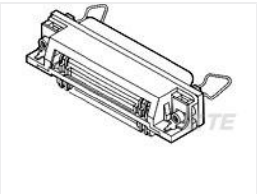
TE Part #5554923-2 RCPT ASSY,SHLD,RTANG, 24 POSN
