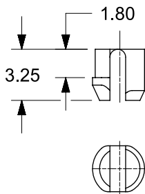
SNAP-FIT PEG
