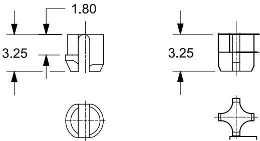
SNAP-FIT PEG
