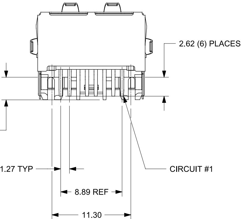
SHIELDING OPTION -B- ENHANCED GROUND TABS
