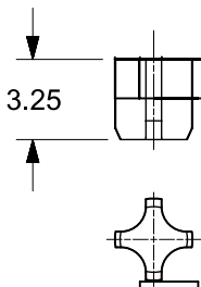
PRESS-FIT PEG
