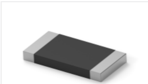
TE Part #6-2176421-8 TLRP 2512 2.0W R082 1% 50PPM 4K RL
