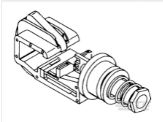
TE Part #58082-1 MTA 156 CRIMP HEAD PRODUCTION POSTED
