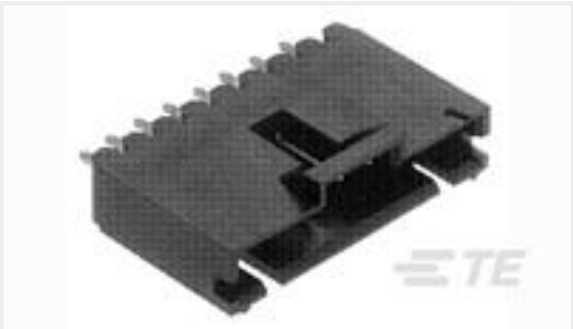
TE Part #7-103639-1 22 MTE HDR SRST LATCH .100CL
