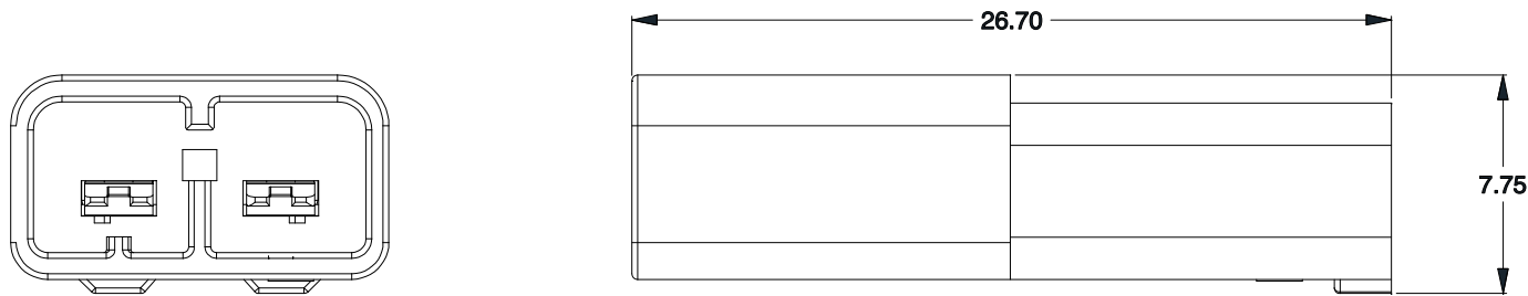
Mated Connector (2271203-1):
