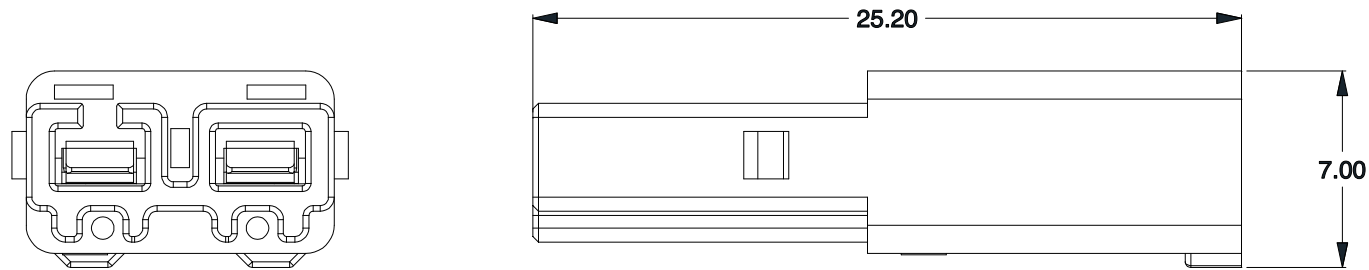
Plug (2271180-1):
