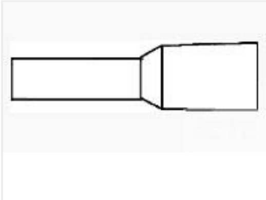
TE Part #1-966293-5 FER,WIRE,PL SLV,1.00/18,L8,RED,HSLP
