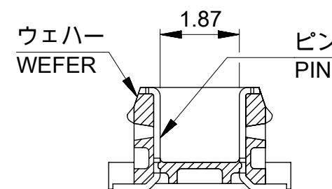
SECT.Z-Z
