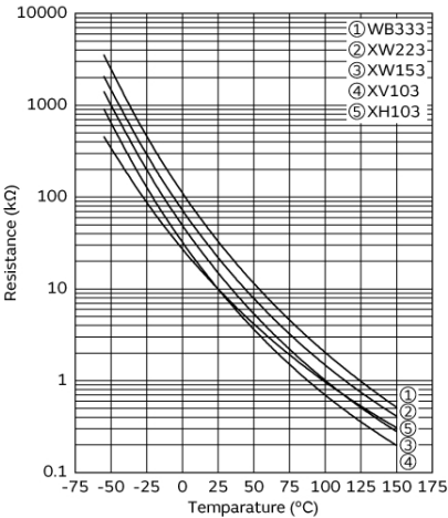
Resistance-Temperature Characteristics
