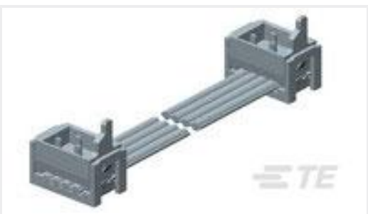
TE Part #2205065-3 CA MICRO-MATCH MOW-MOW 14POS
