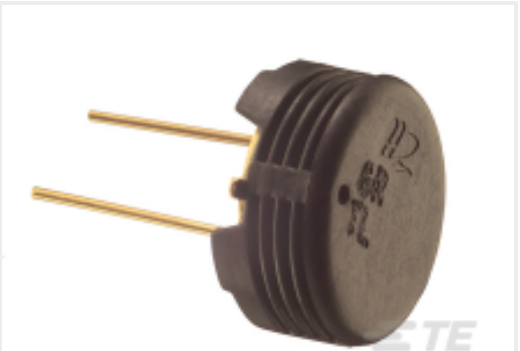
TE Part #HPP801A031 HS1101LF HUMIDITY SENSOR
