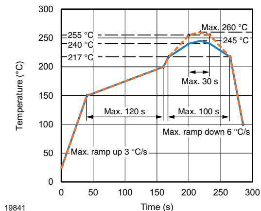
Fig. 8 - Lead (Pb)-free Reflow Solder Profile acc. J-STD-020D
