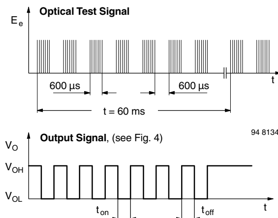
Fig. 3 - Test Signal
