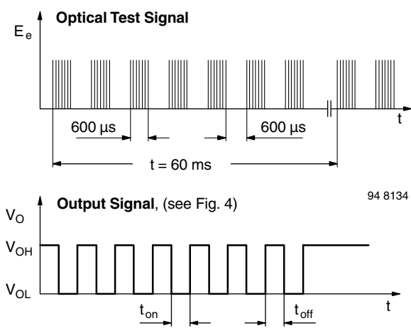
Fig. 3 - Test Signal
