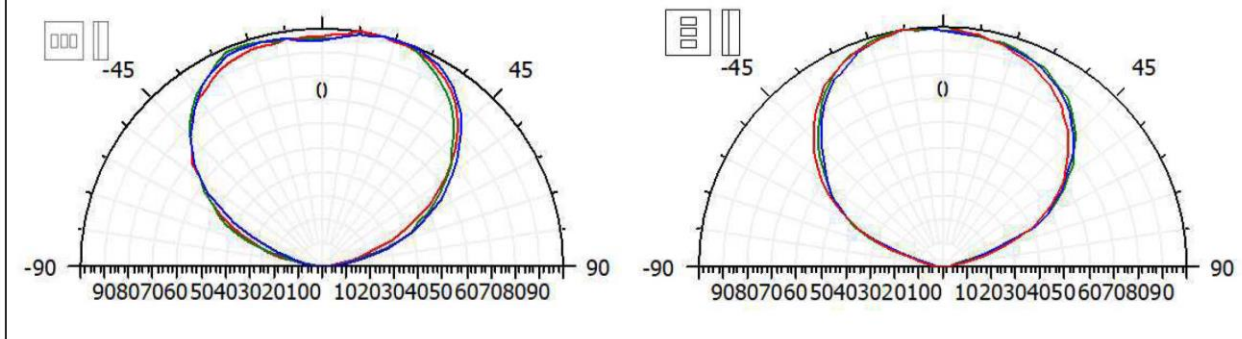
Radiation Diagram(發光角度圖)
