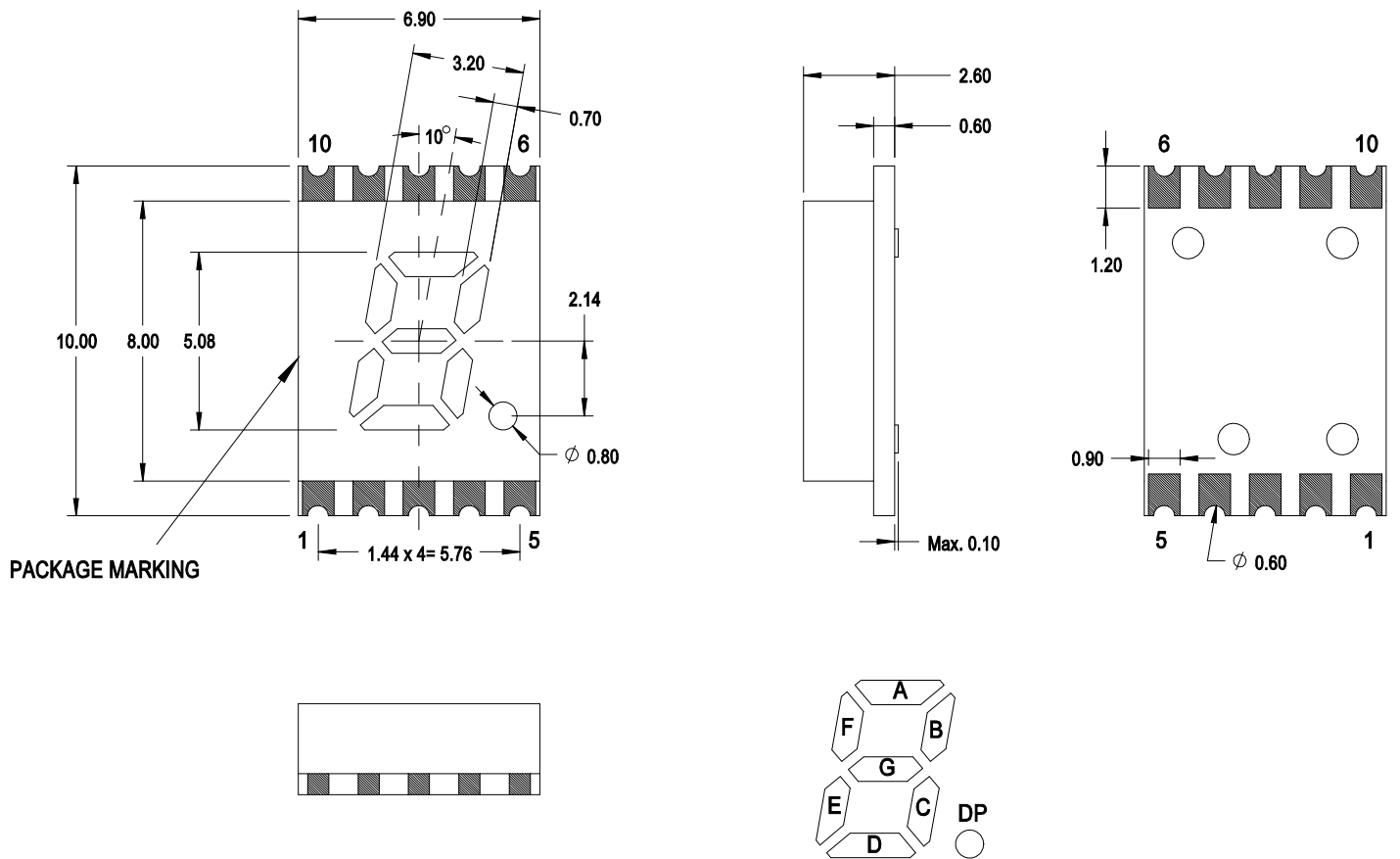
Figure 1: Package Drawing
