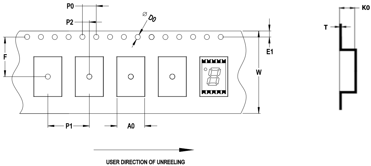
Figure 8: Carrier Tape Dimensions
