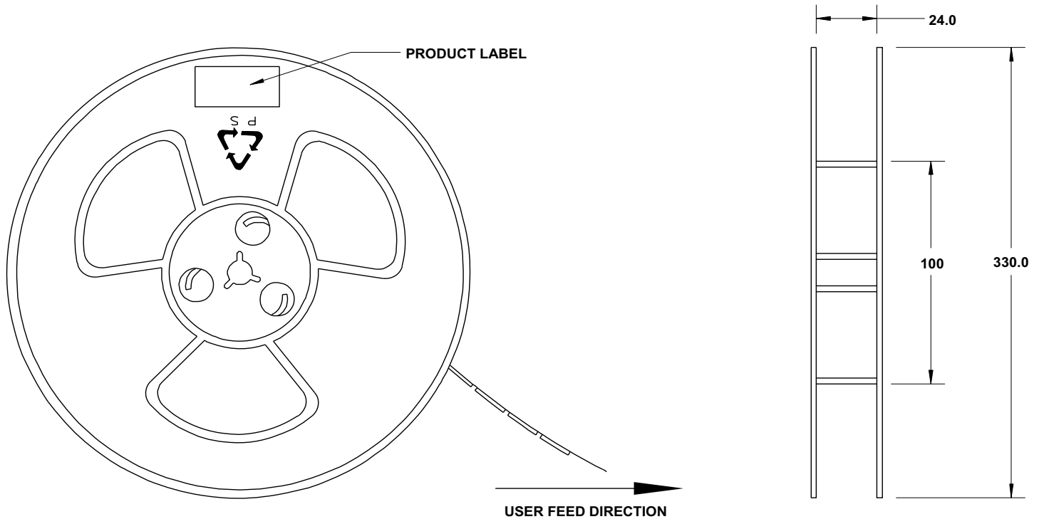
Figure 9: Reel Dimensions
