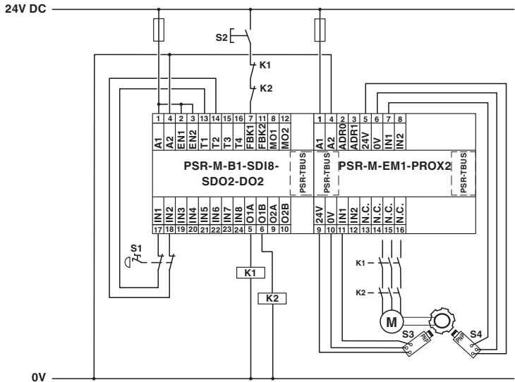
Application drawing
