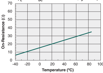
Typical On-Resistance vs. Temperature ( I_L=50mA_{DC} Instantaneous, I_F=5mA )
