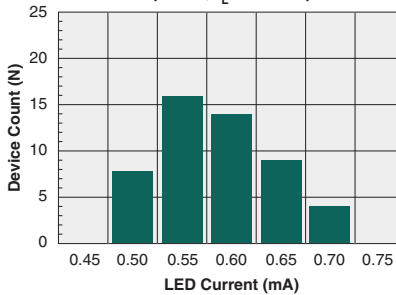
Typical I_F for Switch Operation (N=50, I_L=120mA )
