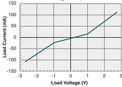
Typical Load Current vs. Load Voltage ( I_F=5mA )
