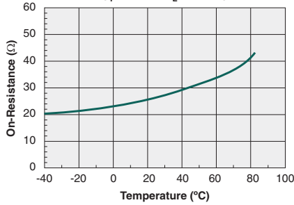
Typical On-Resistance vs. Temperature ( I_F=10mA, I_L=80mA )
