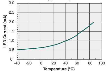
Typical I_F for Switch Dropout vs. Temperature ( I_L=80mA )
