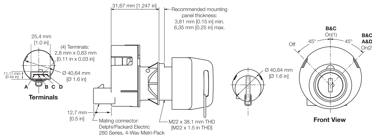
Figure 6. Model 89697 Key Switch Dimensions
