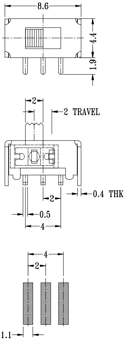
Recommended PCB Layout Top View
