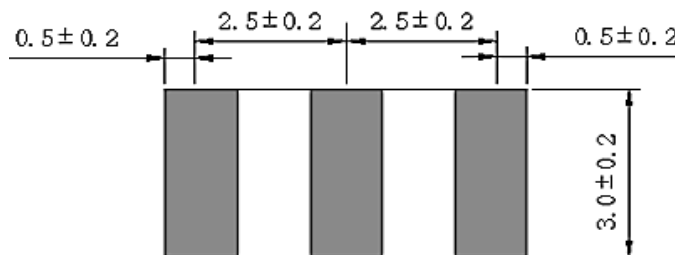
Bottom View
