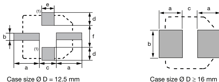
Fig. 4 - Recommended soldering pad dimensions
