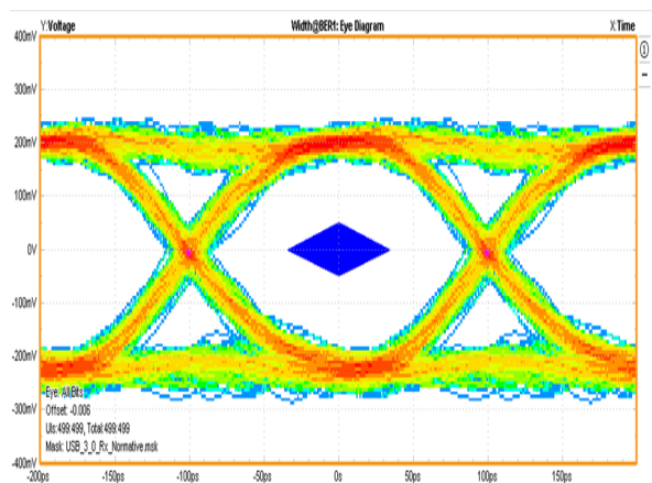
Without ESD8006
