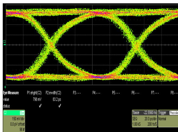
With ESD8006
