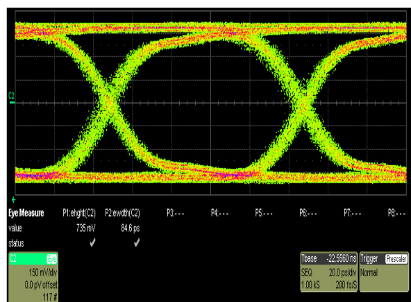
Without ESD8006
