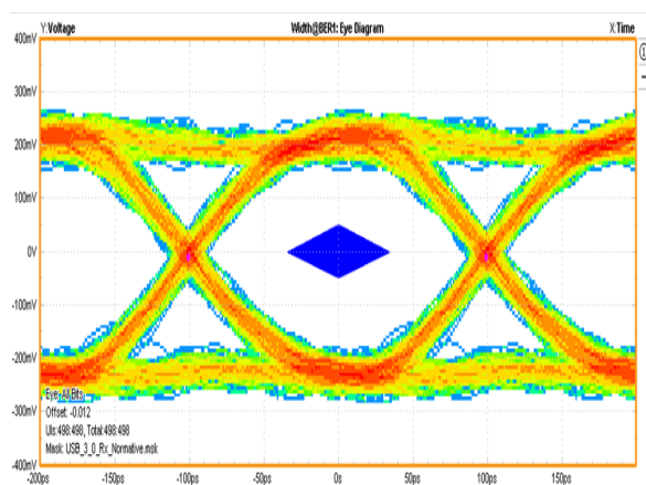
With ESD8006
