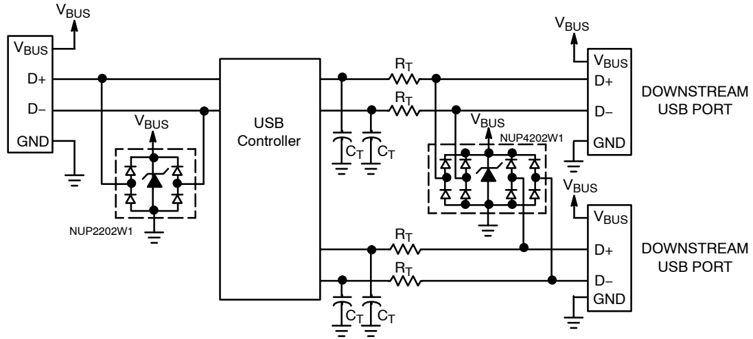
Figure 10. ESD Protection for USB Port
