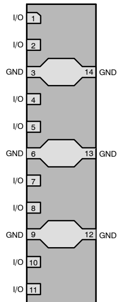
Figure 2. Pin Configuration
