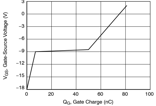
Figure 16. Typical Gate Charge at V_{DS} = 400 \text{ V} and I_D = 24 \text{ A}
