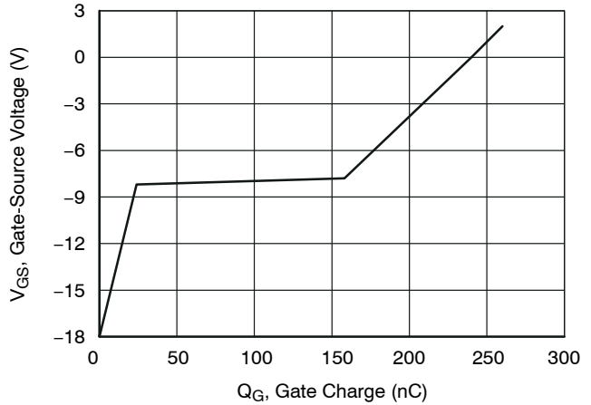
Figure 16. Typical Gate Charge at V_{DS} = 400\text{ V} and I_D = 60\text{ A}
