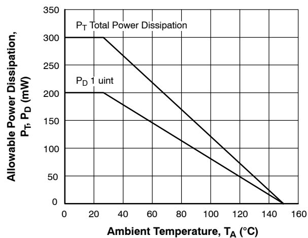
Figure 12. P_T , P_D vs. T_A
