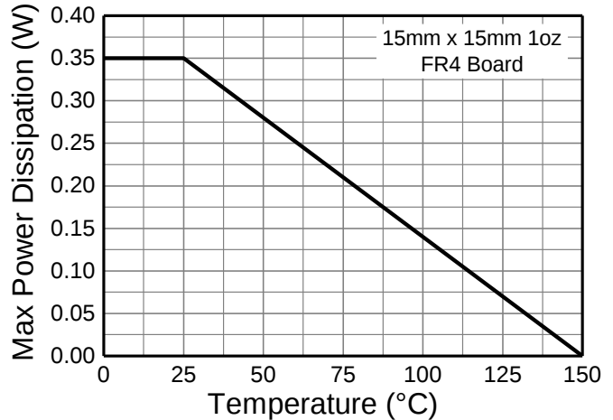
Fig 2. Derating Curve
