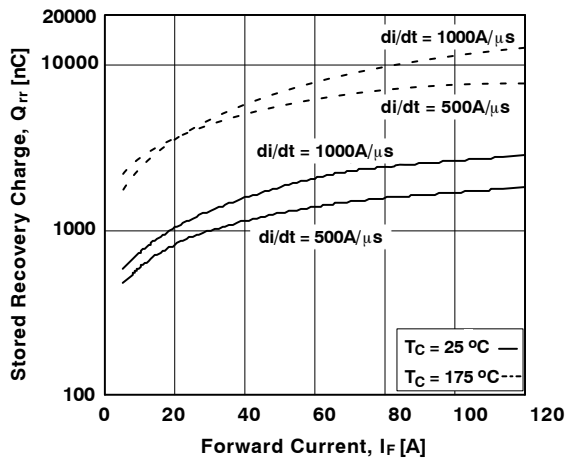
Figure 21. Stored Charge
