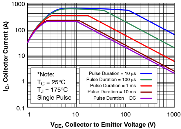
Figure 9. SOA Characteristics
