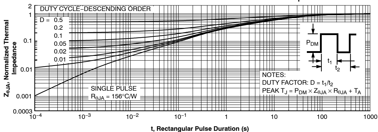
Figure 11. Junction-to-Ambient Transient Thermal Response Curve
