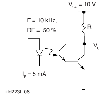
Fig. 6 - Switching Schematic
