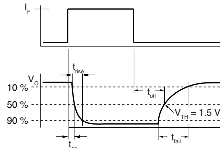
Fig. 7 - Switching Timing
