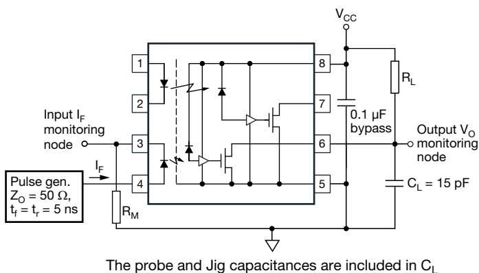
Fig. 1 - Test Circuit for t_{PLH} , t_{PHL} , t_r , and t_f
