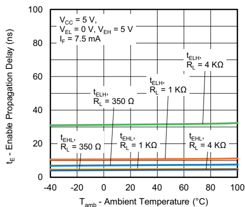
Fig. 13 - Enable Propagation Delay vs. Ambient Temperature
