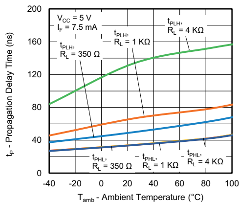
Fig. 12 - Propagation Delay Time vs. Ambient Temperature
