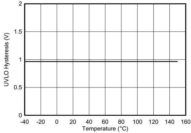
Figure 5-17. VDD 12-V UVLO Hysteresis vs Temperature
