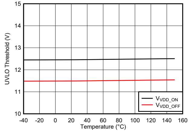
Figure 5-16. VDD 12-V UVLO Threshold vs Temperature
