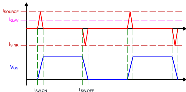
Figure 62. Definition of Current Driving Capability
