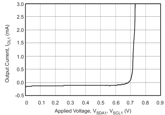
Figure 6-3. Side 1: Output Low Current vs S_{DA1} or S_{CL1} Applied Voltage
